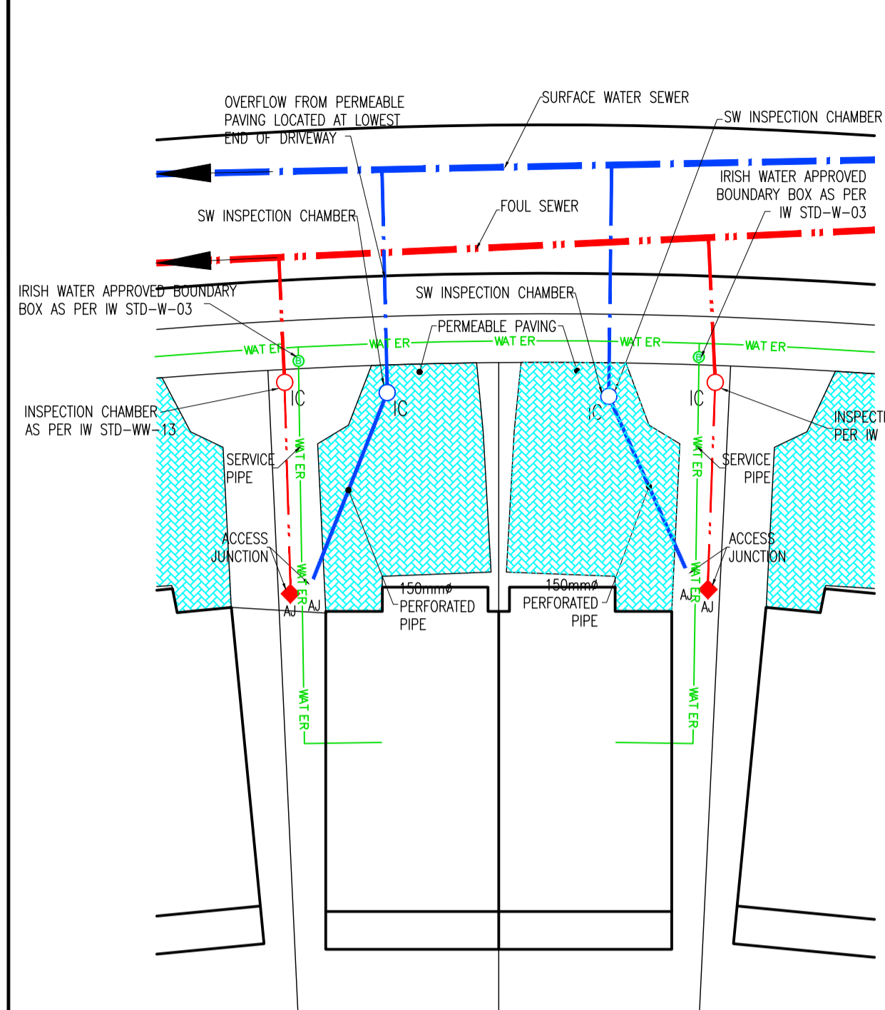
TYPICAL HOUSE DRAINAGE LAYOUT (SEMI-DETACHED) SCALE 1:200
