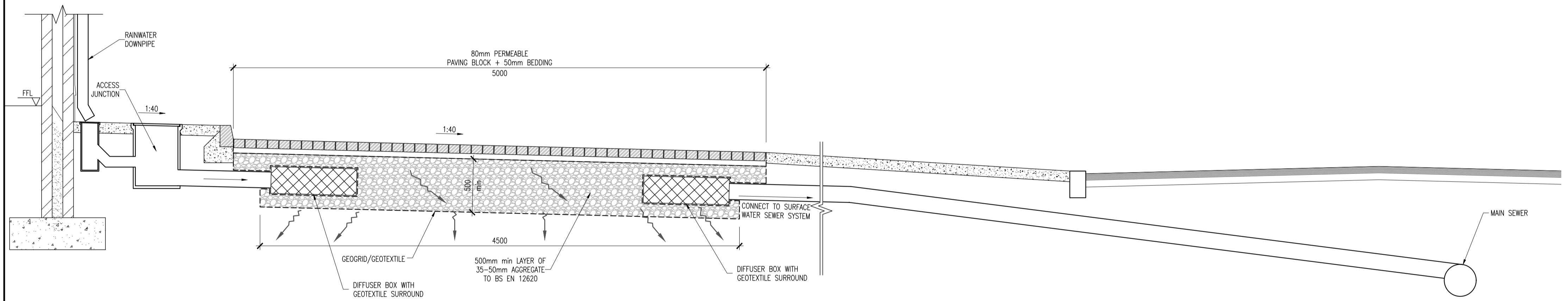
TYPICAL SECTION THROUGH PERMEABLE PAVING DRIVEWAY (WHERE APPLICABLE) SCALE 1:25
