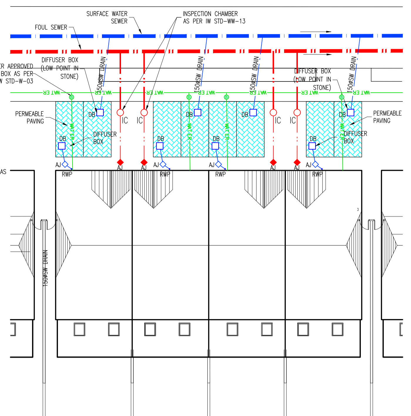
TYPICAL HOUSE DRAINAGE LAYOUT (TERRACED) SCALE 1:200
